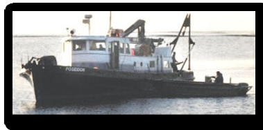
Tug/Utility – Poseidon Length: 64 Ft - Width: 19 Ft - Depth: 8 Ft Horsepower: 180
